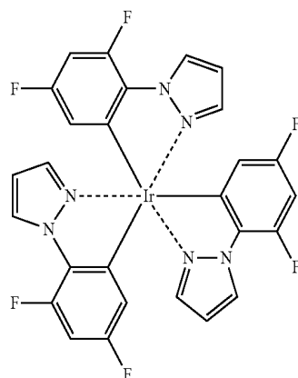
\text{Ir(dfppz)}_3
