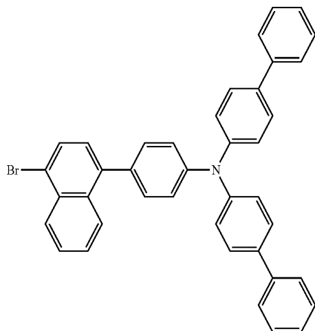
Intermediate 9
