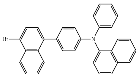
Intermediate 9
