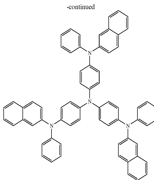
2-TNATA
