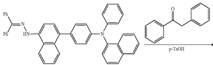
Intermediate 16
