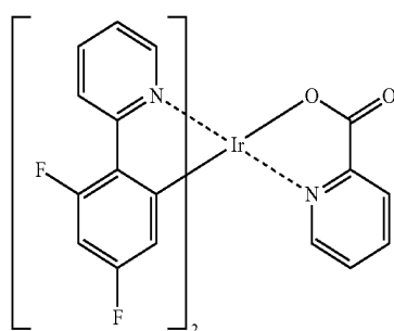
\text{F}_2\text{Irpic}
