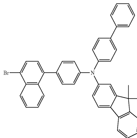
Intermediate 10
