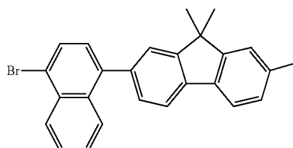
Intermediate 7
