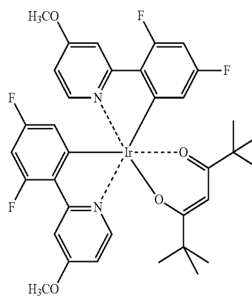
\text{Ir(ppy)}_3
