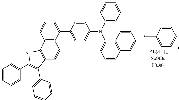
Intermediate 17
